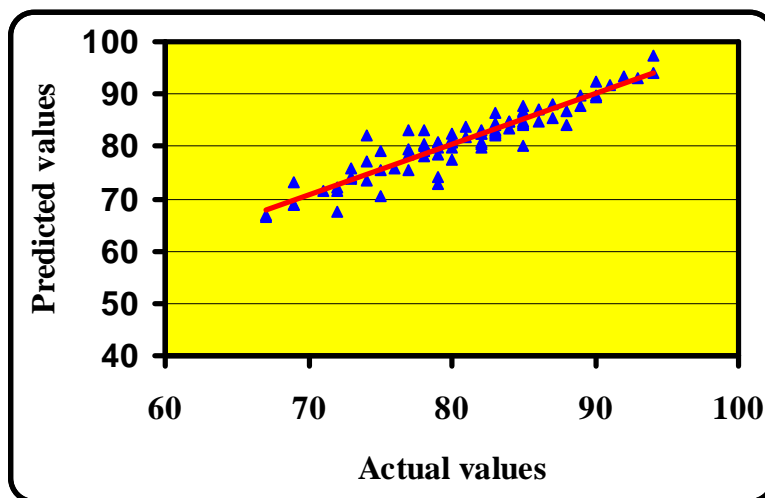
Figure 5: Actual values against the predicted ones using ANN for seam efficiency
