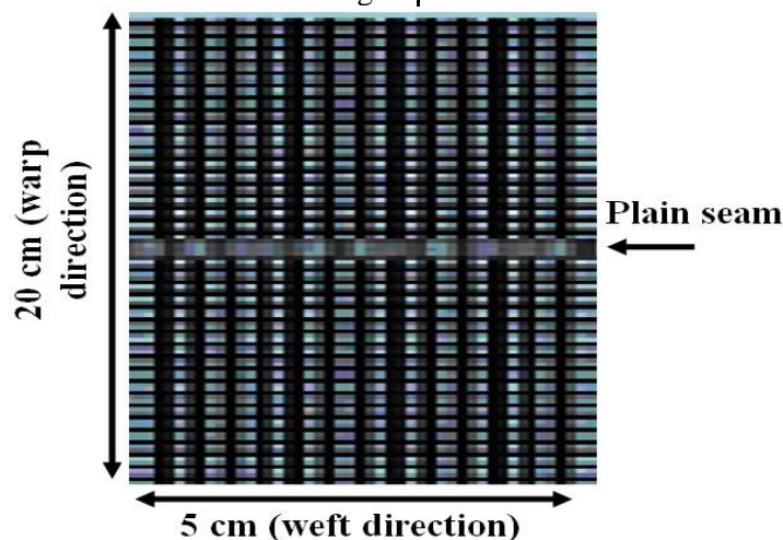
Figure 2: Specimen used to measure seam strength
