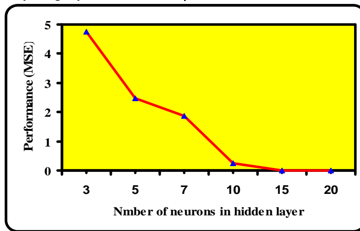
Figure 3: Performance of artificial neural network versus hidden layer neurons' number
