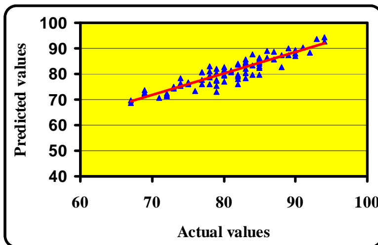
Figure 6: Actual versus predicted values using linear regression for seam efficiency
